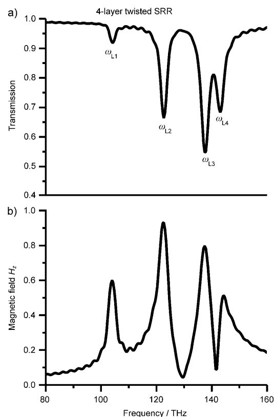
Figure 16. a) Simulated transmission spectrum (L1–L4 = longitudinally coupled split rings) and b) field strength of the H_z component of the four-layer twisted split-ring metamaterial. The probe for the H_z component is positioned at the center of the uppermost split ring. Reprinted from Ref. [42] with permission from the Optical Society of America.
