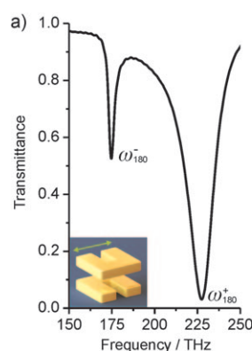
Figure 12. a) Simulated transmittance spectra for the 180°-twisted split-ring dimer metamaterial. The size of each split ring is 230 \times 230 \text{ nm}^2 . The arm width is 90 nm and the gold thickness is 50 nm. The vertical spacing between the two split rings is 50 nm. The structure is embedded in air. The normally incident light is polarized along the gap-bearing side of the top split ring. b) Schematic diagram of the alignments of the magnetic and electric dipoles in the two split rings at the respective resonance frequencies. The solid and dashed arrows represent the magnetic and electric dipole moments, respectively. Reprinted from Ref. [38], with permission from the Nature Publishing Group.
