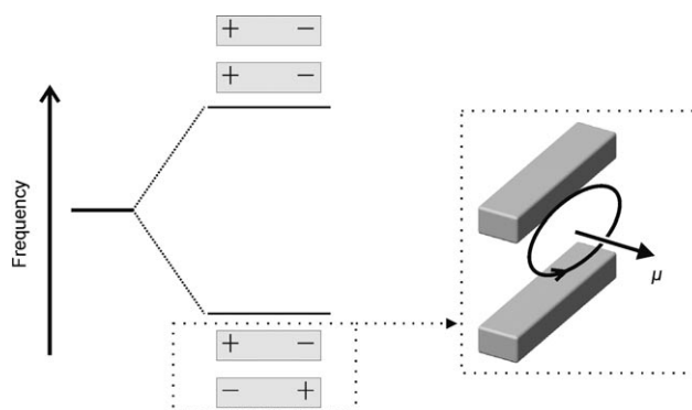
Figure 4. Transverse coupling of two coupled metallic nanowires. A magnetic dipole moment can be excited in the antisymmetric mode and acts as a magnetic “atom”.
